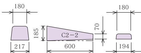
C両R～C両R(2段下り-2) H=70
