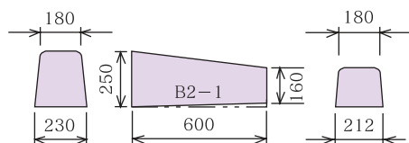
B両R～B両R(2段下り-1) H=70
